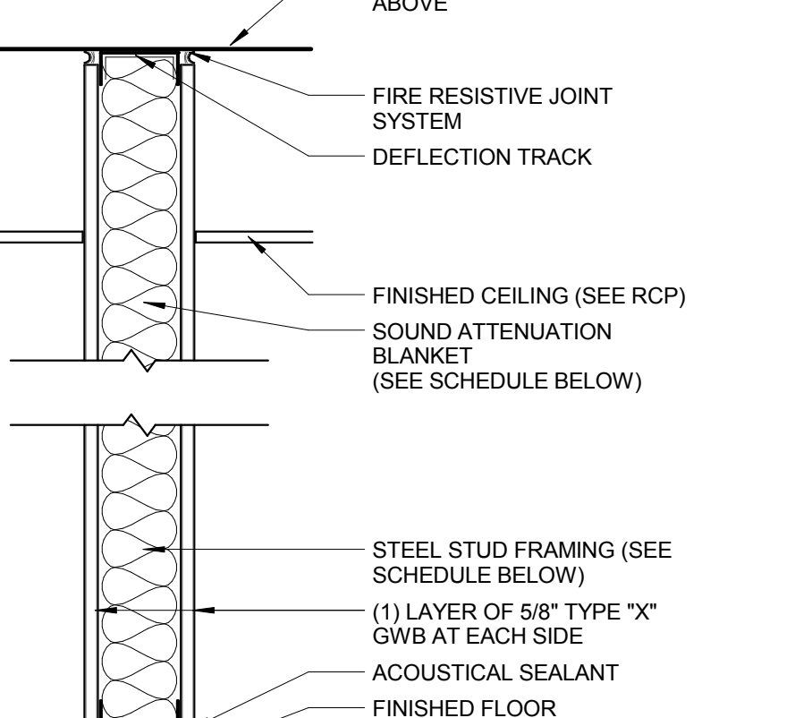
1 HR RATED PARTITION SCALE: 1 1/2" = 1'-0" UL DESIGN U465
