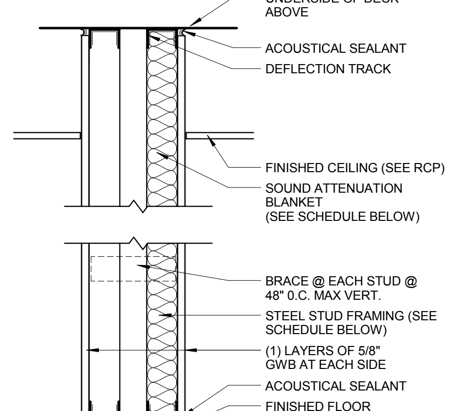
NON-RATED SOUND PARTITION SCALE: 1 1/2" = 1'-0"
